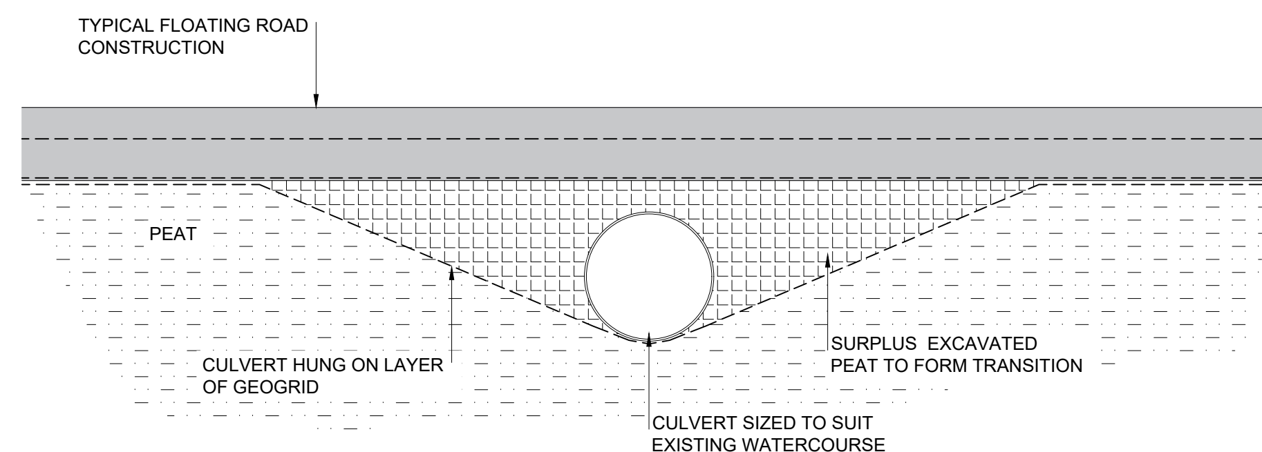
FLOATING ROAD CULVERT DETAIL SCALE 1:50
