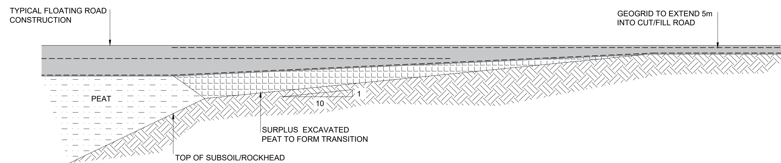
FLOATING ROAD TO CUT/FILL TRANSITION DETAIL SCALE 1:50
