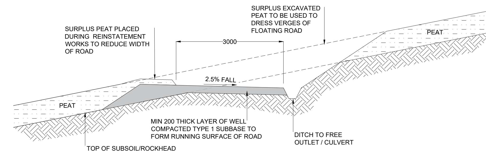
TYPICAL SECTION THROUGH CUT/FILL ROAD AFTER CONSTRUCTION PERIOD SCALE 1:50
