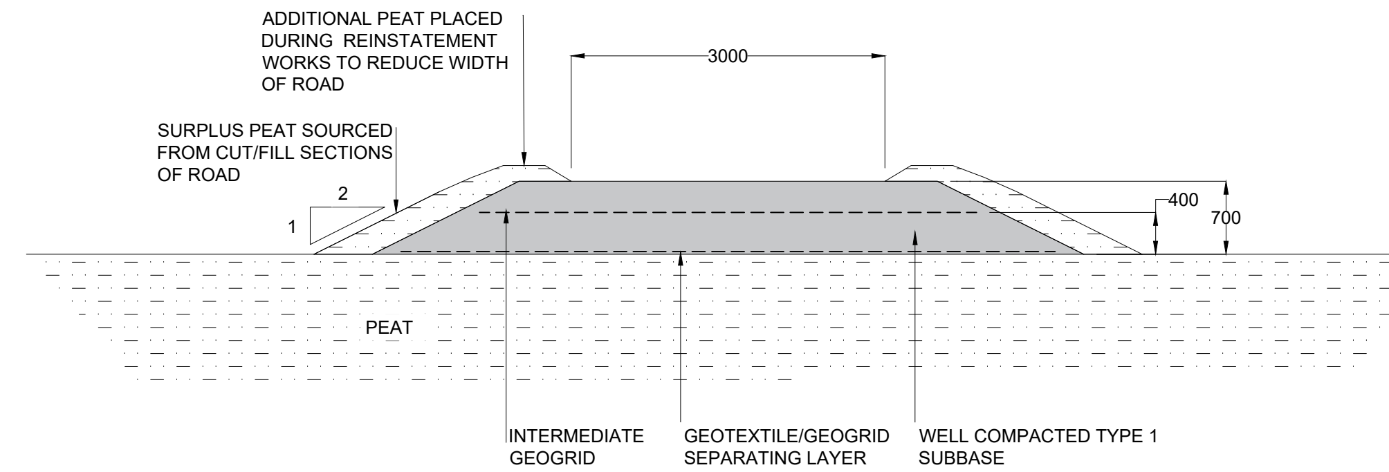
TYPICAL SECTION THROUGH FLOATING ROAD AFTER CONSTRUCTION PERIOD SCALE 1:50
