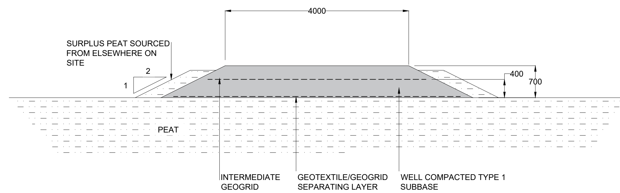
TYPICAL SECTION THROUGH FLOATING ROAD DURING CONSTRUCTION PERIOD SCALE 1:50
