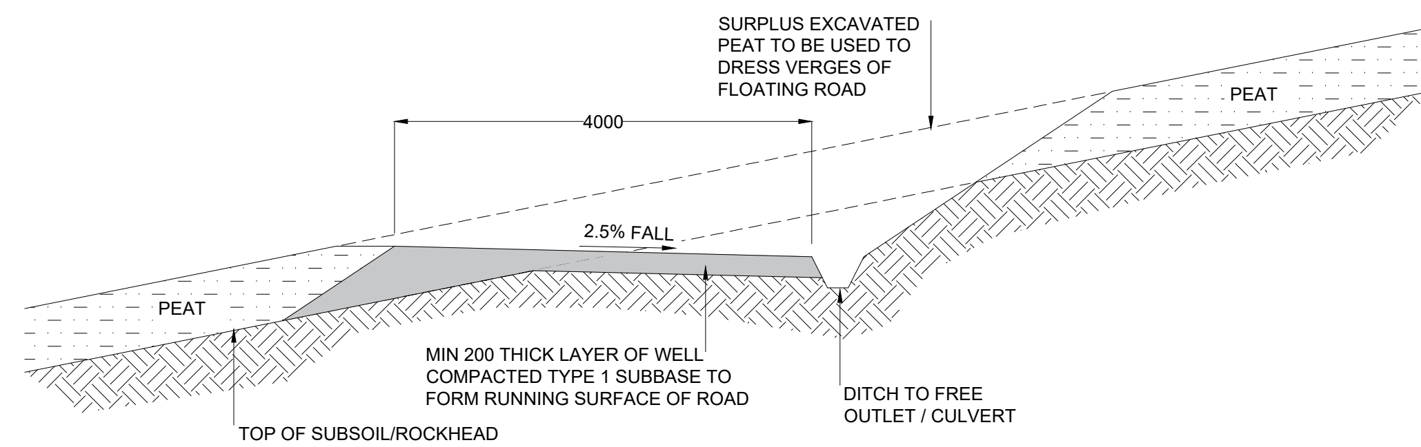
TYPICAL SECTION THROUGH CUT/FILL ROAD DURING CONSTRUCTION PERIOD SCALE 1:50
