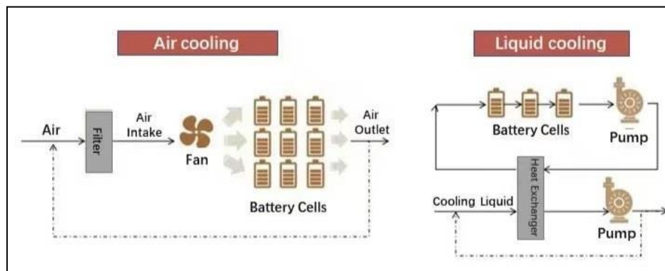
Figure 2. Air-cooled System vs Liquid Cooled System
