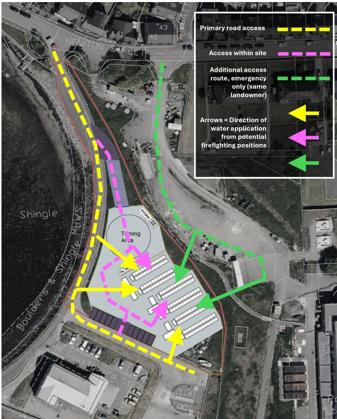
Figure 4. Firefighting Approach Plan.
