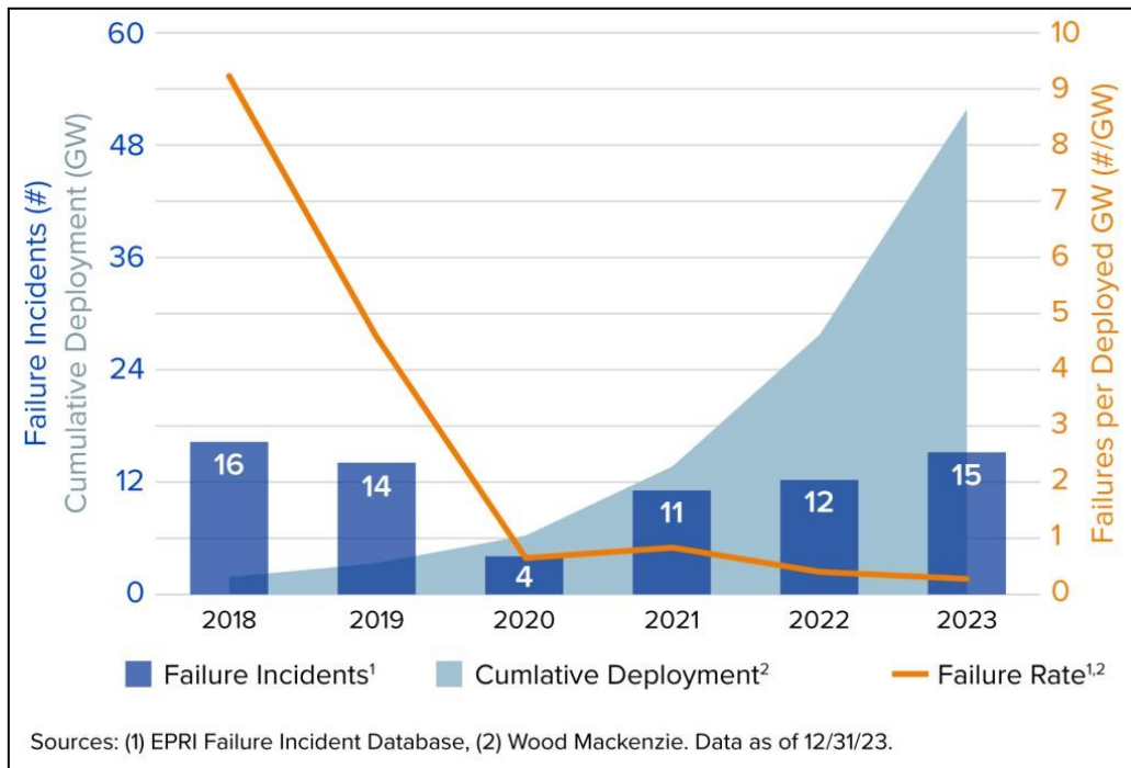
Figure 3. Global Grid-Scale BESS Deployment and Failure Statistics, Source EPRI.
